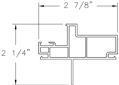
MAIN FRAME FIN INSTALLATION (BP4003) EXTRUDED RIGID PVC
