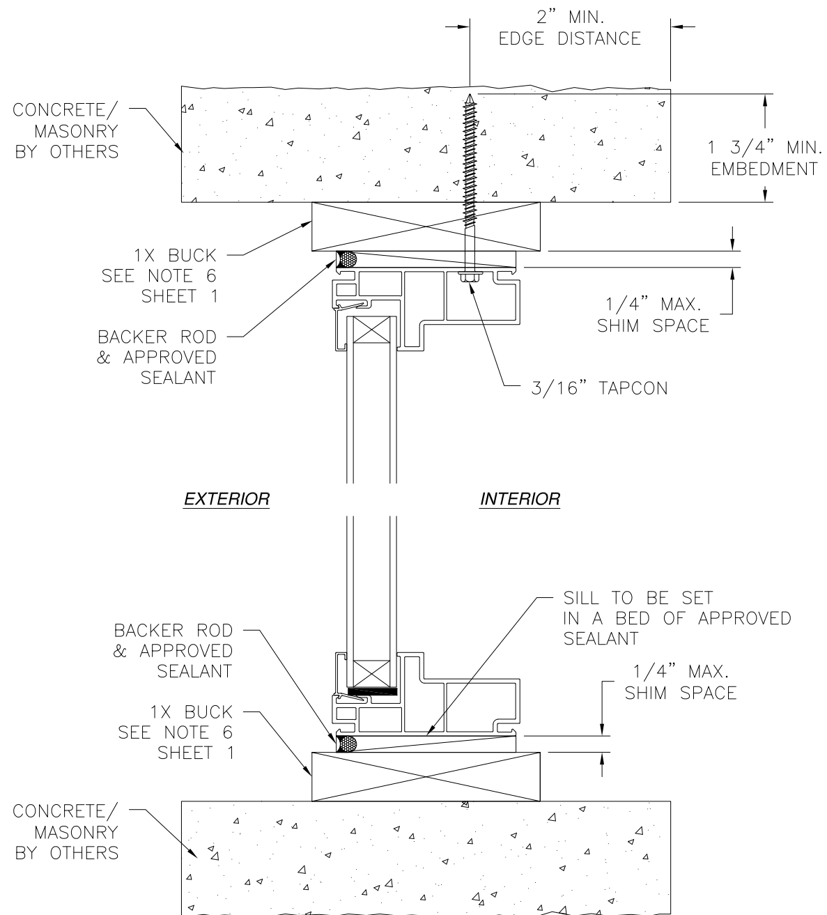
VERTICAL CROSS SECTION CONCRETE/MASONRY WITH 1X BUCK INSTALLATION FOR CONCRETE/MASONRY INSTALLATION WITHOUT 1X BUCK REFER TO JAMB INSTALLATION DETAILS
