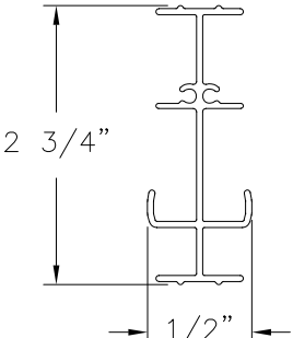
COMMON JAMB REINFORCEMENT (208A) ALUMINUM 6063-T5
