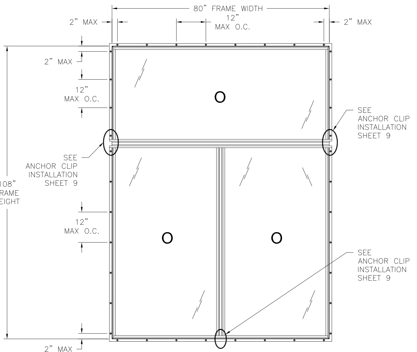
SERIES 400/475 TWIN PICTURE WINDOW W/TRANSOM EXTERIOR VIEW FIN INSTALLATION
