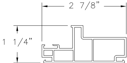
MAIN FRAME (BP4003) EXTRUDED RIGID PVC
