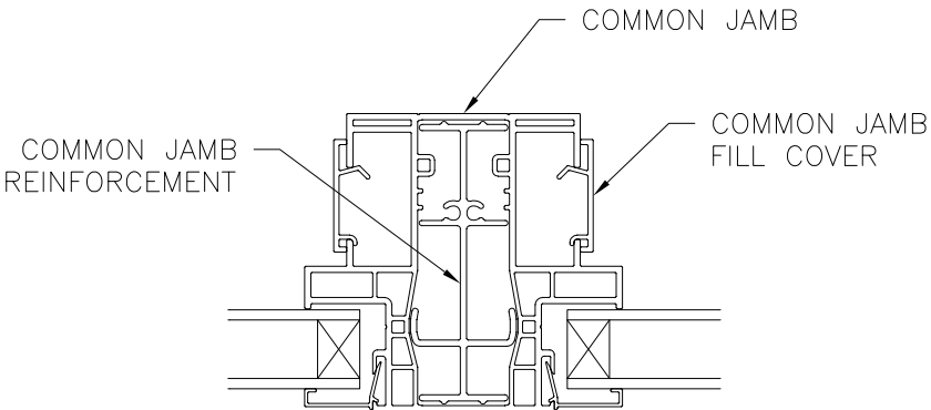
VERTICAL MULLION
