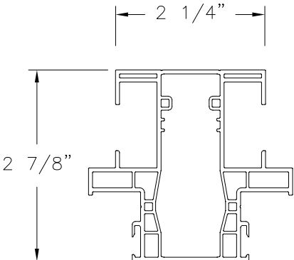
COMMON JAMB (BP4010) EXTRUDED RIGID PVC
