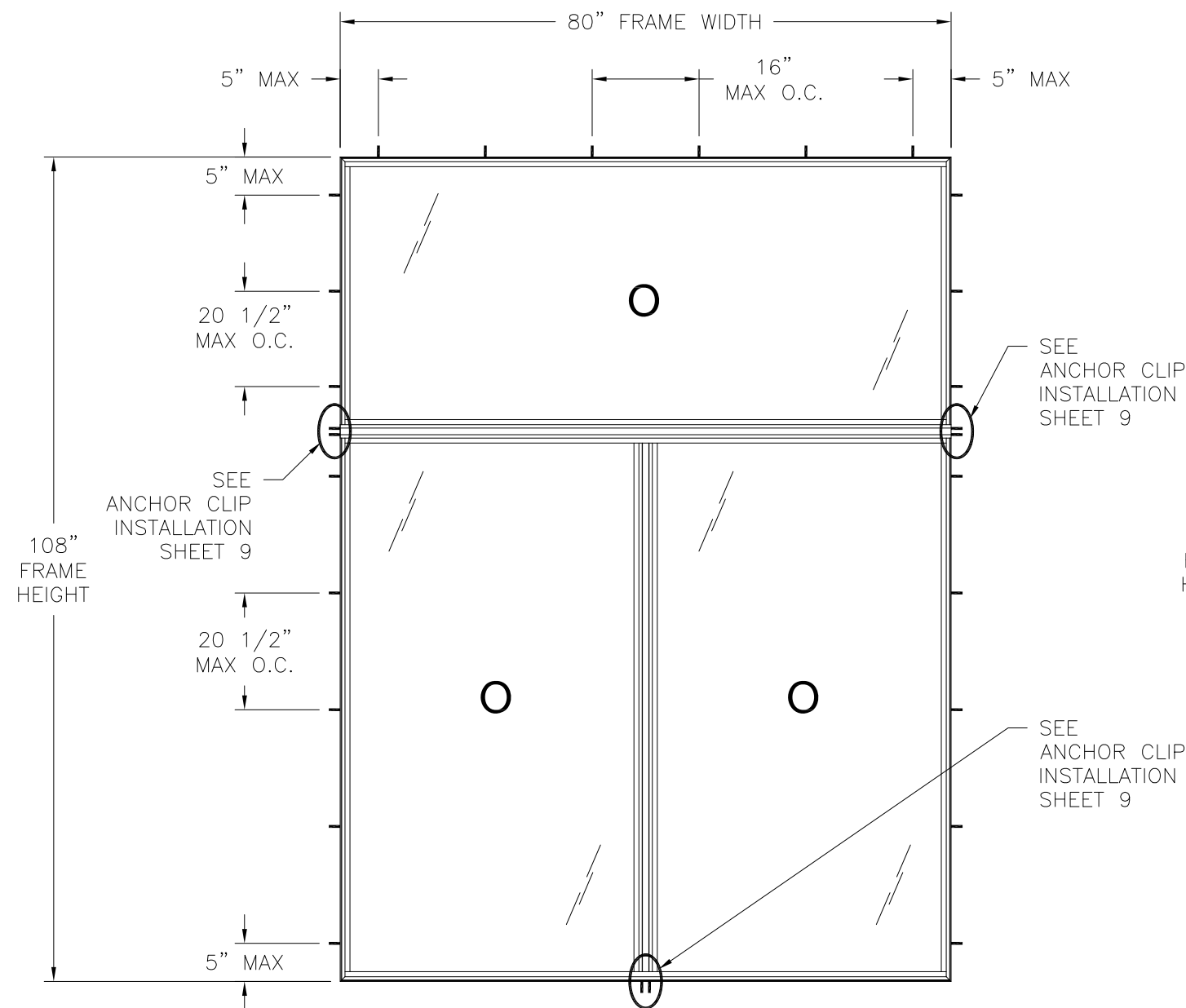
SERIES 400/475 TWIN PICTURE WINDOW W/TRANSOM EXTERIOR VIEW FRAME INSTALLATION
