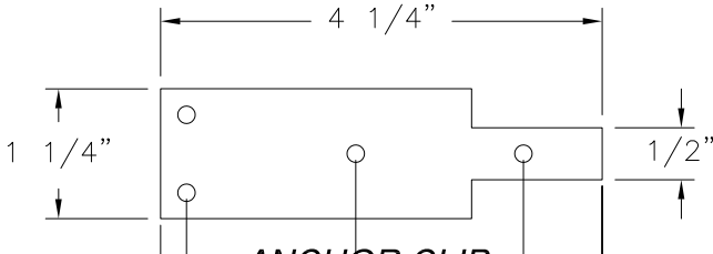
ANCHOR CLIP ALUMINUM 6061-T6
